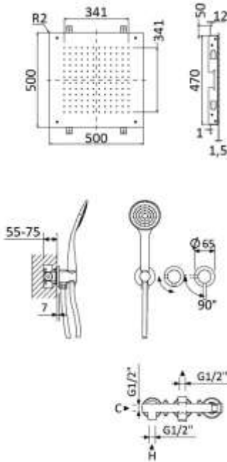
DIAGRAMA CAUDAL | FLOW DIAGRAM
