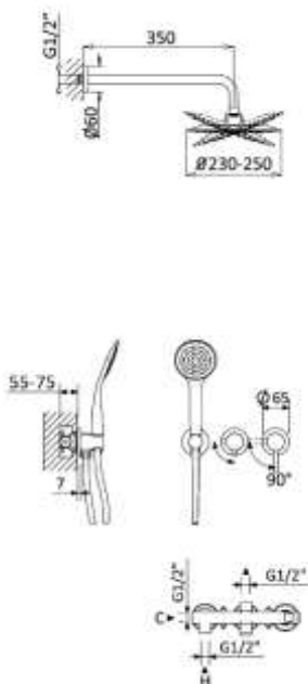
DIAGRAMA CAUDAL | FLOW DIAGRAM
