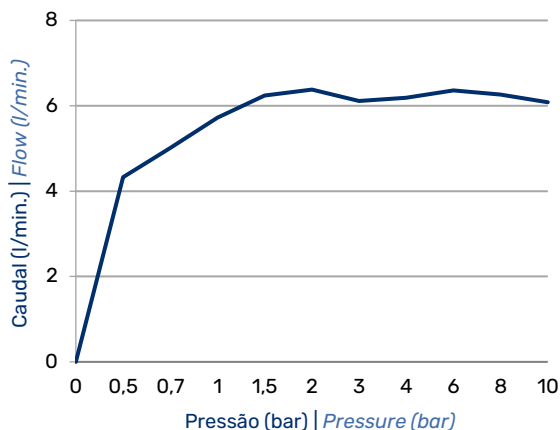
DIAGRAMA CAUDAL | FLOW DIAGRAM
