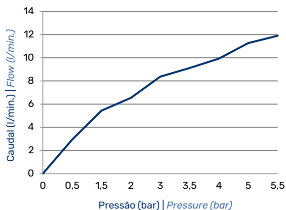
DIAGRAMA CAUDAL | FLOW DIAGRAM
