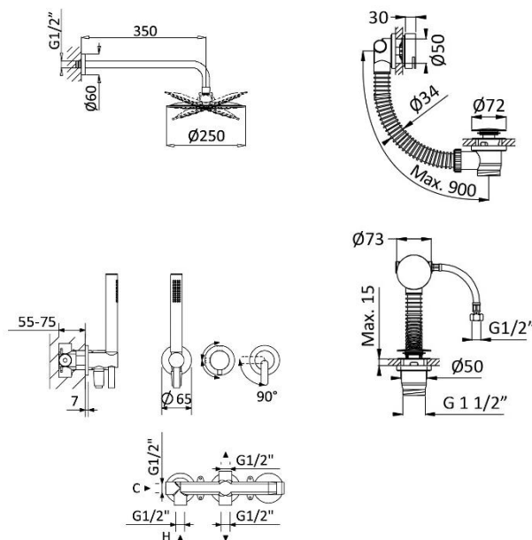
DIAGRAMA CAUDAL | FLOW DIAGRAM
