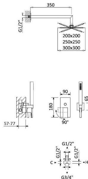
DIAGRAMA CAUDAL | FLOW DIAGRAM
